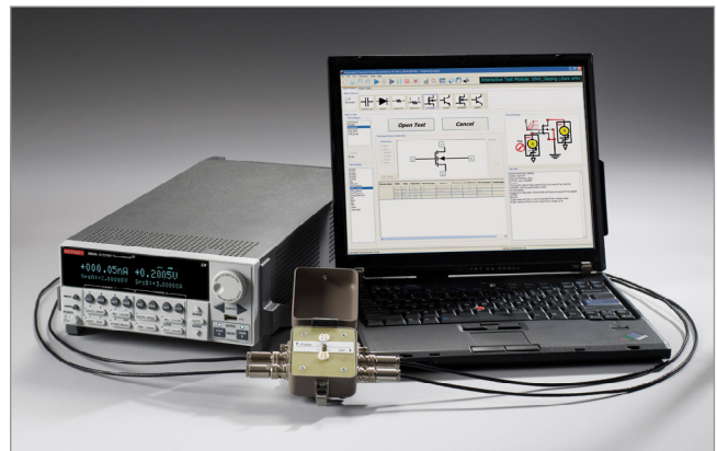
The flexible software architecture of ACS Basic Edition allows configuring systems with a wide range of controllers and test fixtures, as well as the exact number of SourceMeter SMU instruments the application requires.
